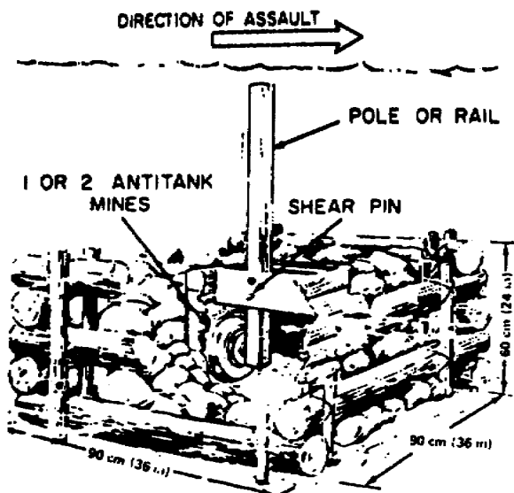
Figure 3-28. Nutcracker.
